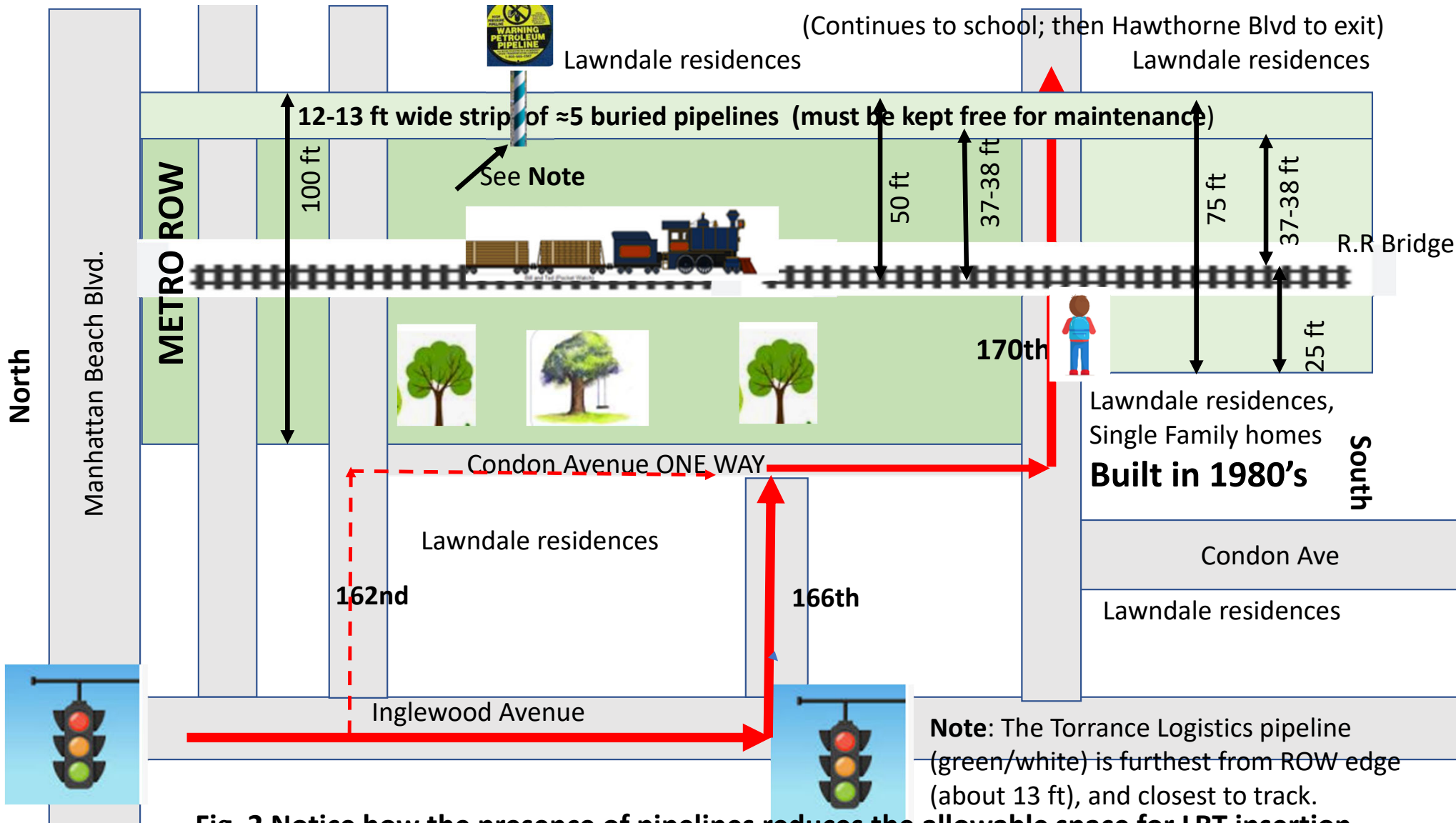
Fig. 2 Notice how the presence of pipelines reduces the allowable space for LRT insertion.
